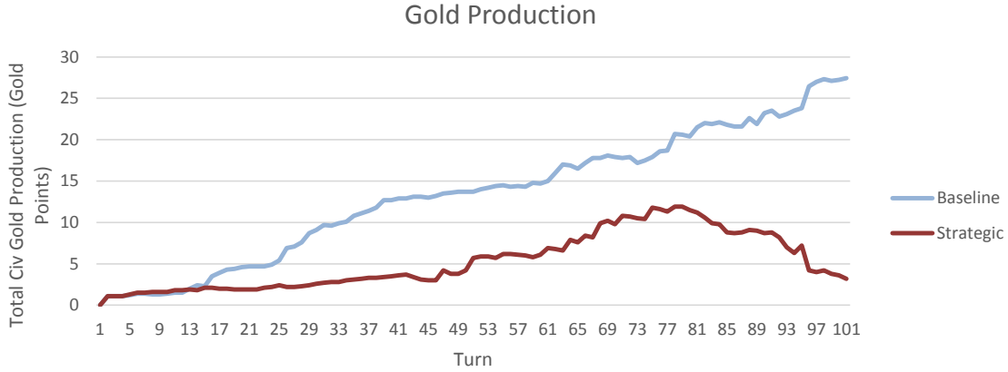
Figure 11. Gold production rate with and without strategies for resolving tradeoffs
