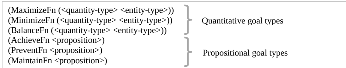
Figure 2. Vocabulary of goal types.
