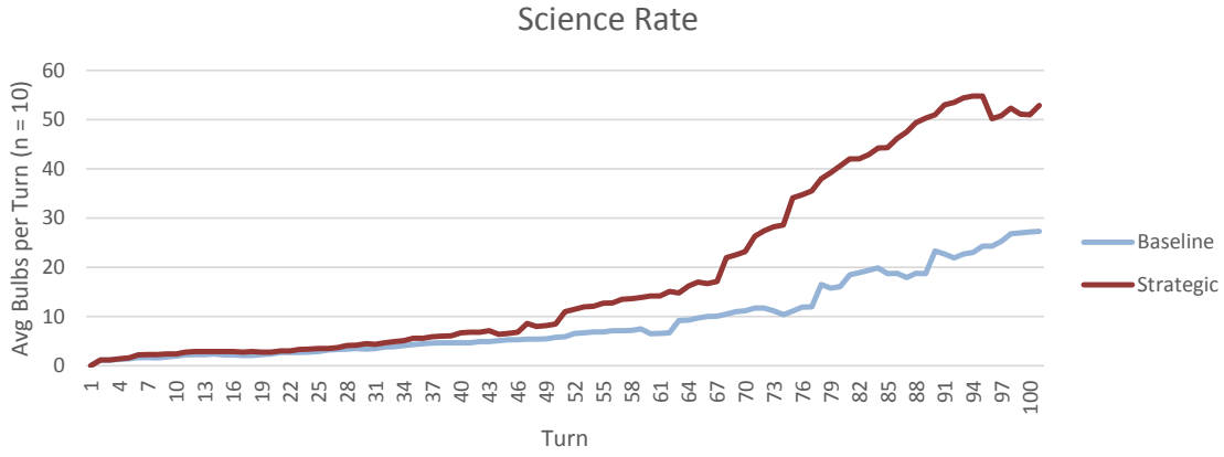
Figure 10. Science output rate with and without strategies for resolving tradeoffs
