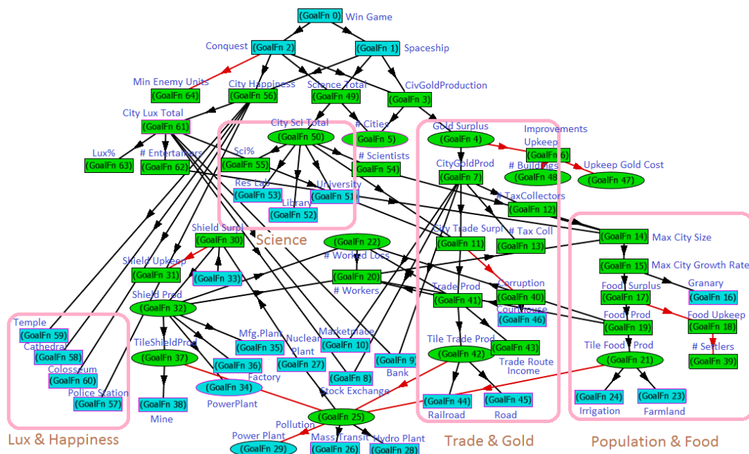
Figure 5: A Freeciv goal network, based in part on learned knowledge of the game.
